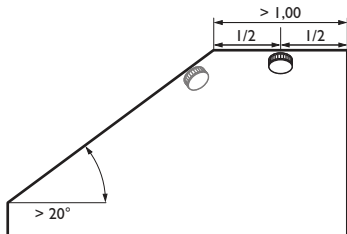
Fig. 13 Straight mounting surface at least 1 m long and 1 m wide
