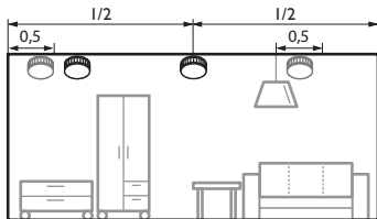
Fig. 11 Rooms with straight ceilings
